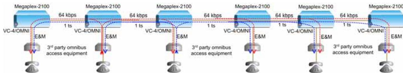
Figure 5. Typical Point-to-Multipoint (Omnibus) Connection
